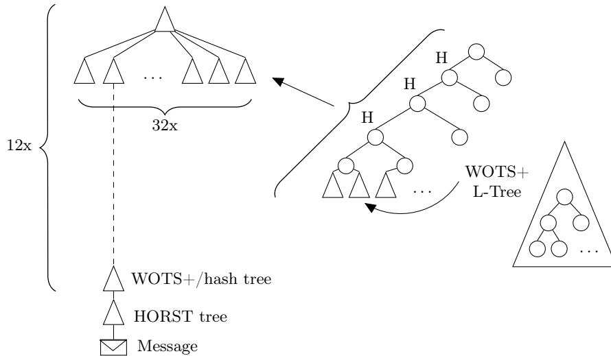
Fig. 4. The complete hypertree structure
